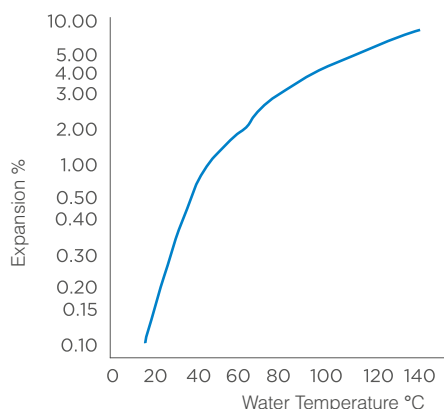
Water Expansion According To Temperature Difference
