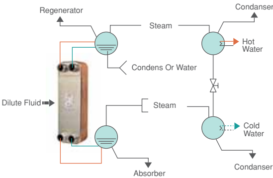
Absorbed Refrigeration
