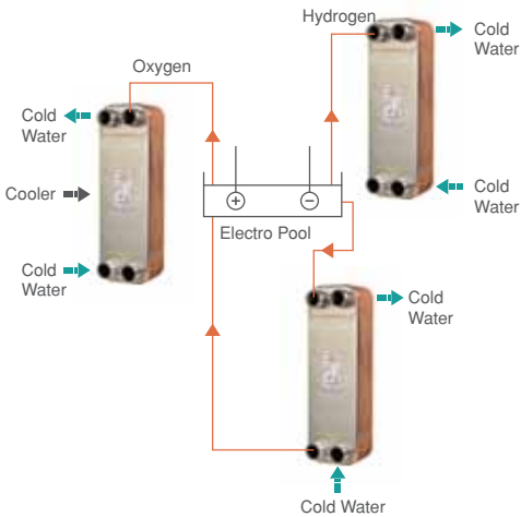
Electrolysis Process Circuit
