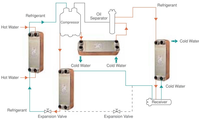
Cooling System Circuit (Refrigerant)
