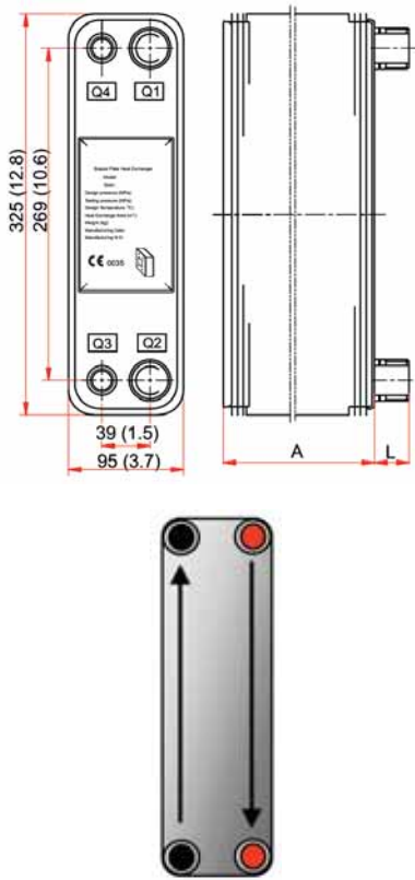
Parallel Flow
