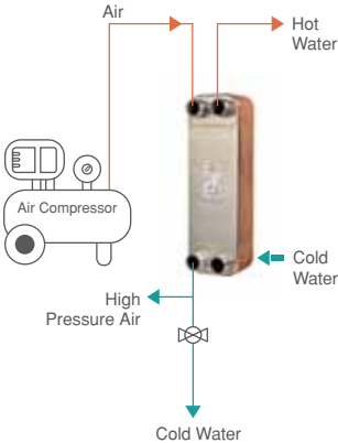
Air-Drying Cooler
