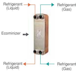
Economizer
