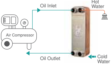
Heat Recovery (Compressor)
