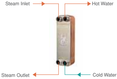
Domestic Hot Water System With Steam
