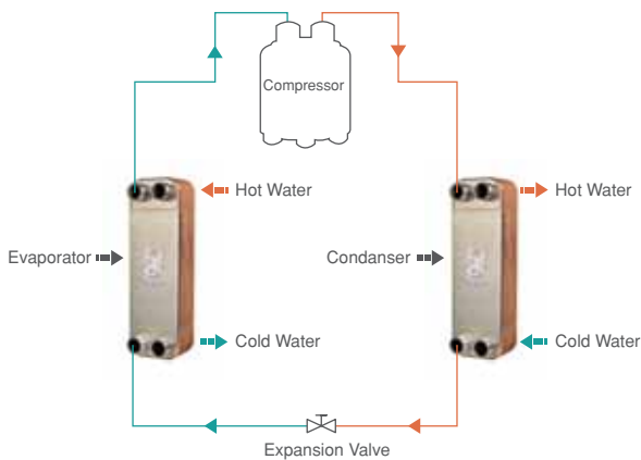
Refrigeration (Water Source)
