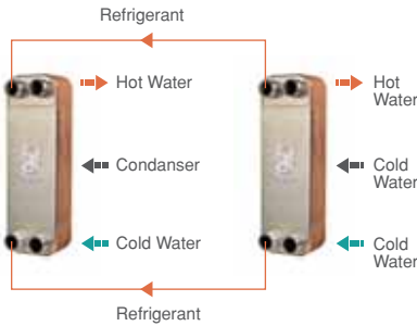
Pre Cooler
