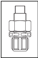
Fig. 5: WT Injection fitting
