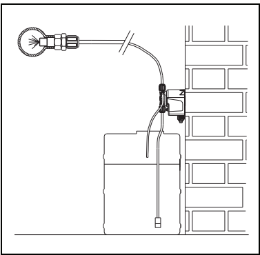
Fig. 11: Wall mounted installation
