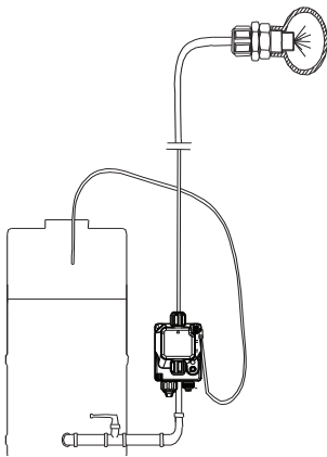
Fig. 12: Flooded suction mounting
