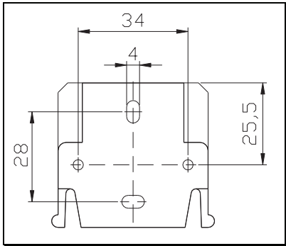
Fig.8 Bracket drilling template
