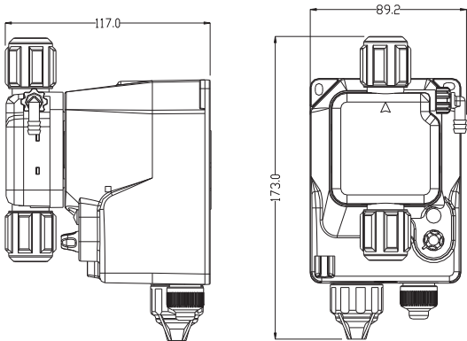
Fig.7 Overall dimensions of pump
