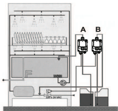
Fig. 10: Installation on a dishwashing machine
