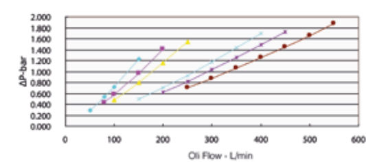
Oil Pressure Loss Performance
