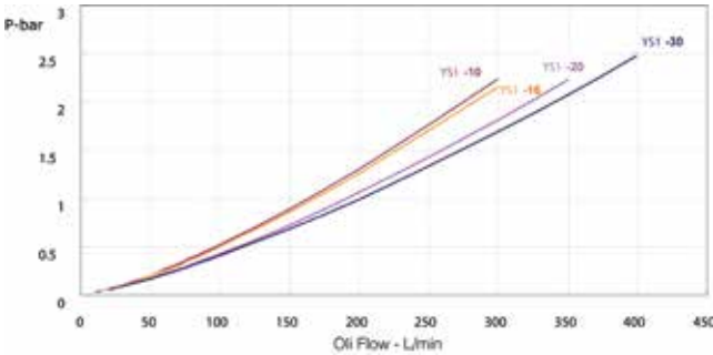
Pressure (YS1-10)->(YS1-30)
