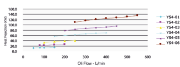
Heat Rejection (YS4-01)->(YS4-06)
