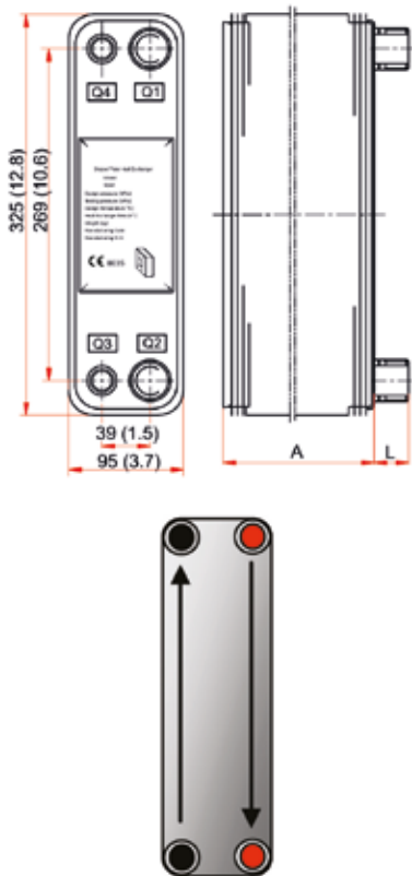
Parallel Flow
