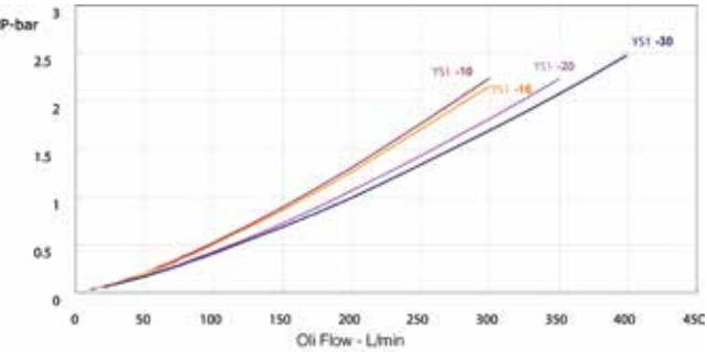
Specific Heat Rejection (YS1-10)->(YS1-30)
